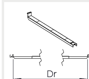
Omega/ALG2 railbracket (4)
