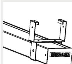
9905215 Omega / ALG2 safety suspensionrail bracket 110
