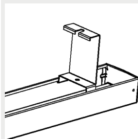
9905216 Omega / Alfa Line G2 Ladderbracket
