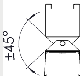
9905201 Gamma/Eco S adjustable suspension rail 120 bracket
