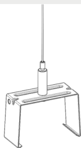
G00342 Gamma/Eco S suspension wire bracket 5m
