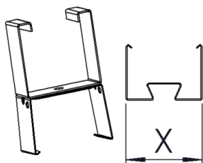
3508171 Gamma/Eco S suspension rail 70 bracket
