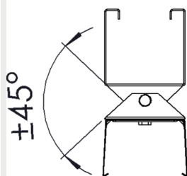
9905200 Gamma/Eco S adjustable suspension rail 70 bracket
