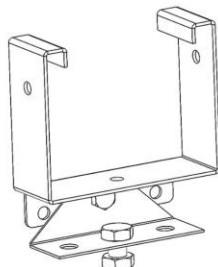
E 1500227 Origi MEK 82 adjustable End cap bracket
