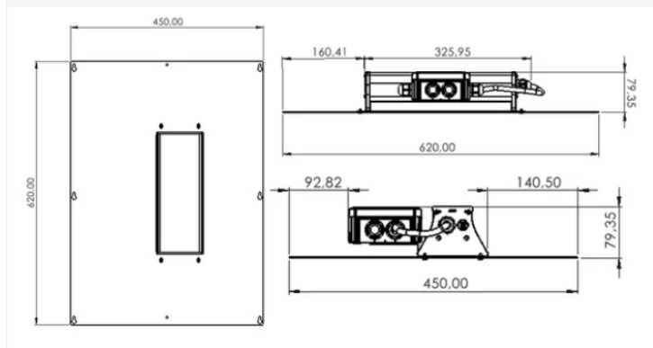
Underpass- E1500267 Origi Canopy recessed frame
