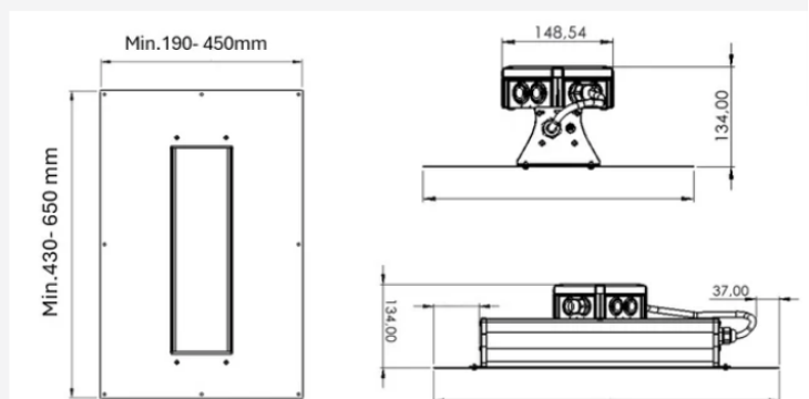
Origi Canopy tailor recessed frame
