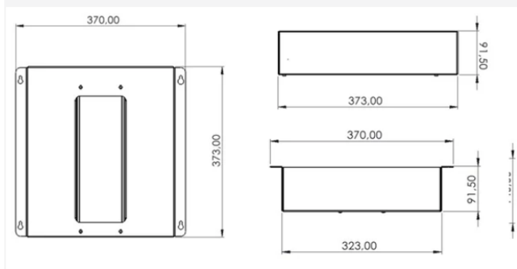
E1500271 Origi Canopy surface mounting frame
